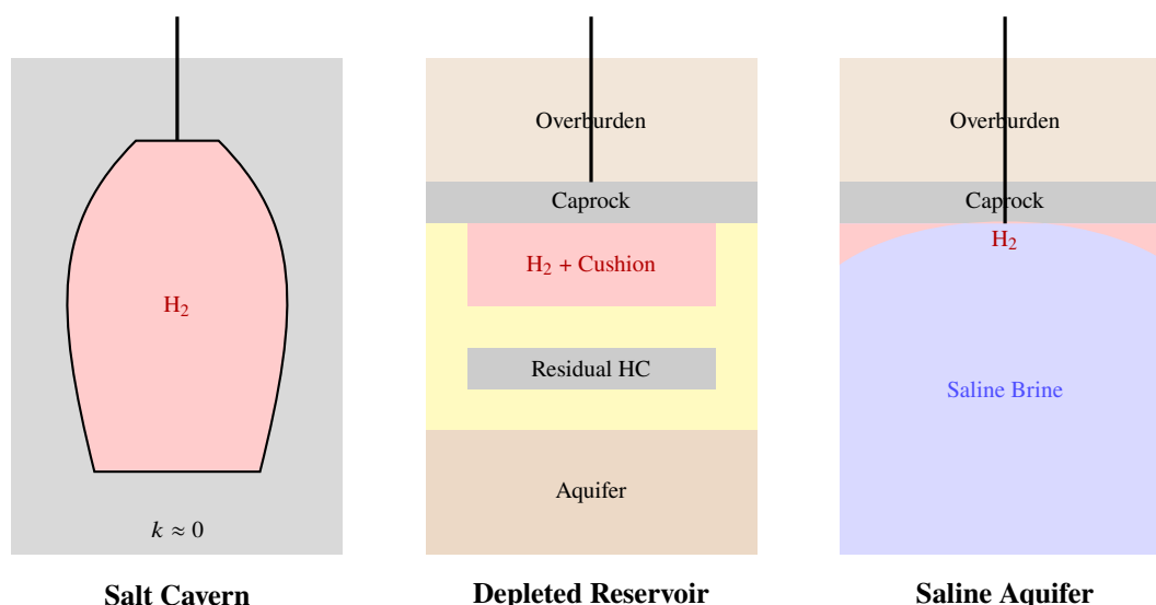
Figure 1. Schematic comparison of the three primary geological formation types for underground hydrogen storage.
