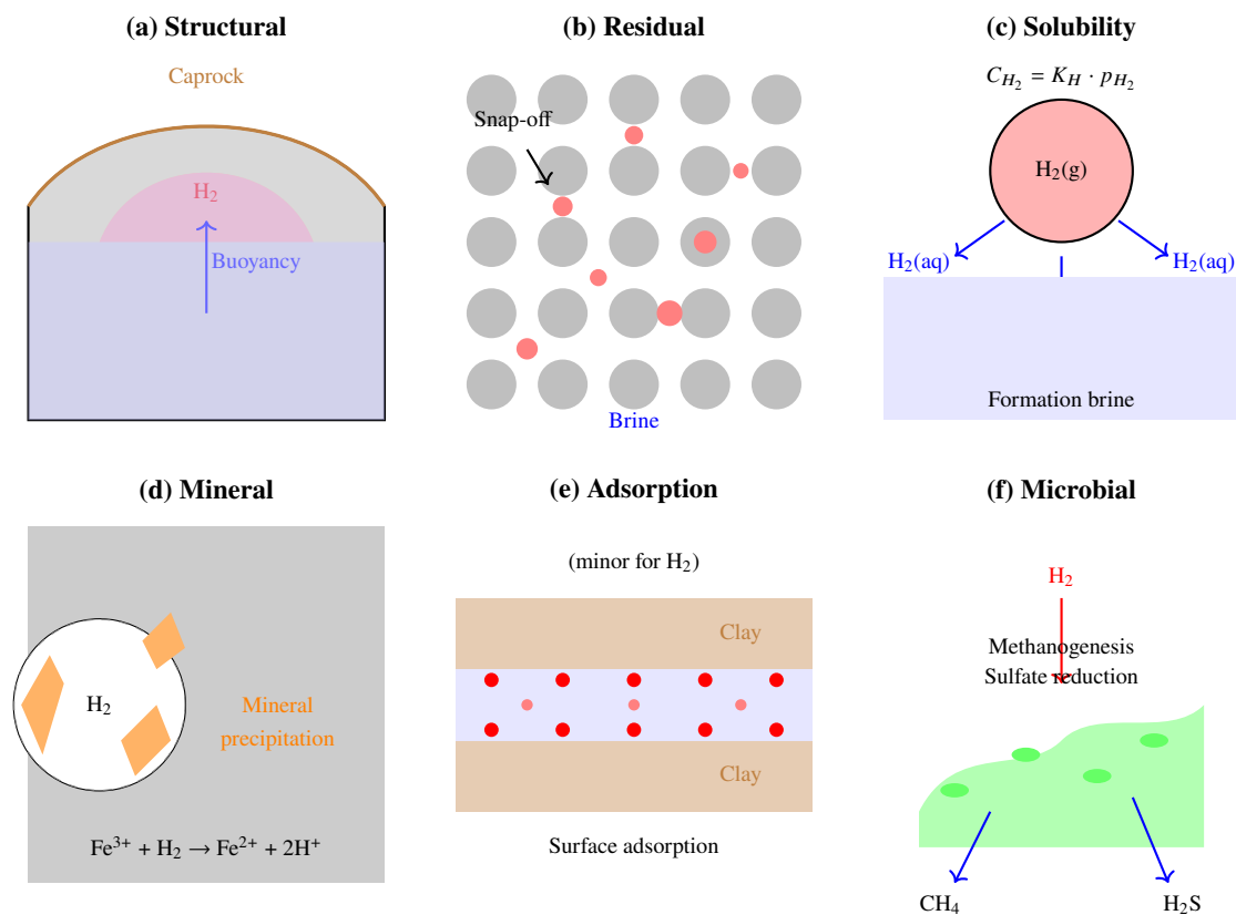
Figure 3. Schematic representation of hydrogen trapping mechanisms in underground storage: (a) structural trapping beneath low-permeability caprock driven by buoyancy; (b) residual trapping of disconnected gas ganglia following snap-off during imbibition; (c) solubility trapping via dissolution into formation brine governed by Henry's law; (d) mineral trapping through geochemical reactions (typically minor for H_2 ); (e) adsorption on mineral surfaces (minor contribution); (f) microbial consumption converting H_2 to CH_4 or H_2S . Structural and residual trapping dominate storage security; solubility and microbial mechanisms represent loss pathways.
