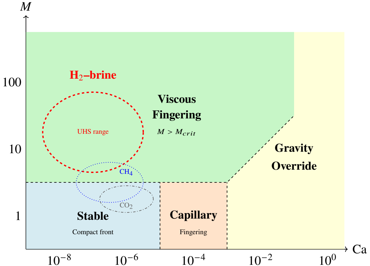
Figure 2. Multiphase flow regime map in capillary number–mobility ratio ( \text{Ca} – M ) space for gas–brine displacement in porous media. Hydrogen–brine systems (red dashed ellipse) typically operate in the viscous fingering regime due to high mobility ratios ( M \sim 20\text{--}100 ), in contrast to \text{CH}_4 and \text{CO}_2 systems that may achieve more stable displacement. Regime boundaries are approximate and depend on pore structure and wettability.
